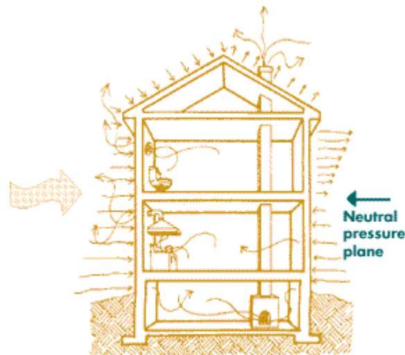
Forces causing air leakage
