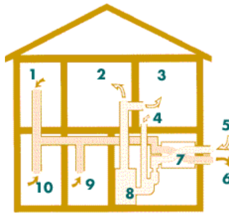
Schematic of ventilation system with an HRV
